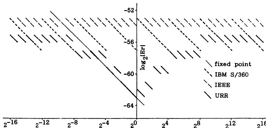
Fig.1 Relative Error(Er), with 64 bits data.
